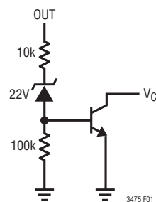
Figure 1. External Overvoltage Protection Circuitry for the LT3475-1
